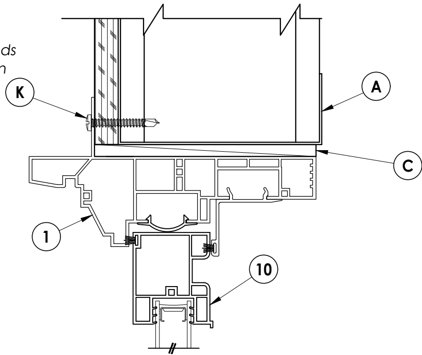
2 VERTICAL CROSS SECTION 3 Shown w/ Steel Stud framing option
