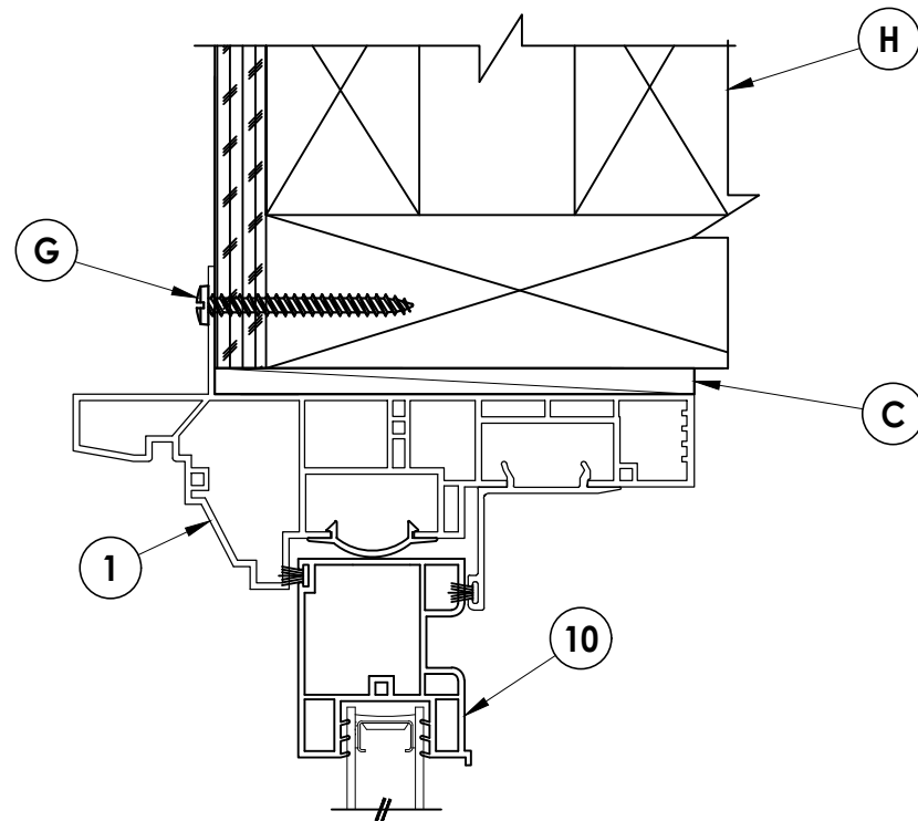
1 VERTICAL CROSS SECTION 3 2x Stud Construction
